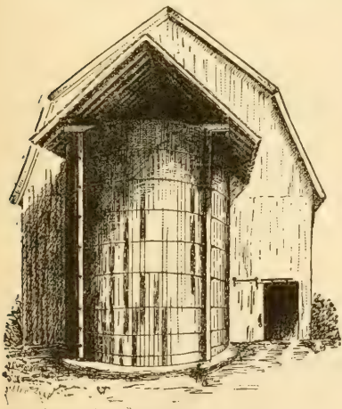
FIG. 178. A cheap roof of stave silo. (Clinton.)
